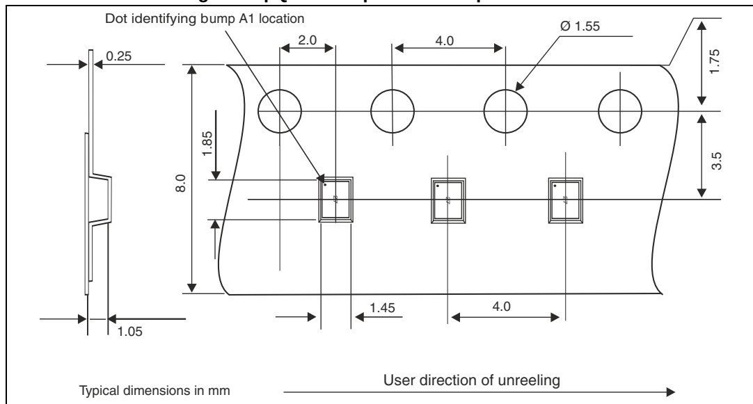
Figure 10. Flip Chip tape and reel specification
